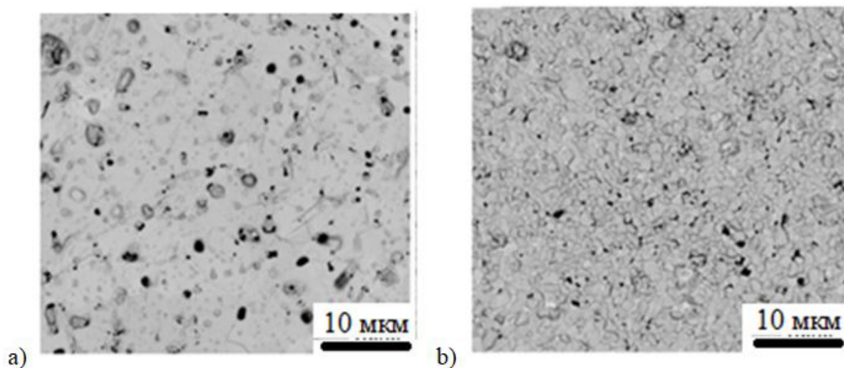
Figure 2: SEM micrographs of barium (a) and strontium (b) cobaltites obtained by melt quenching in a solar furnace. The temperature dependence of resistivity ( \rho ) and samples are shown in Fig.3.
