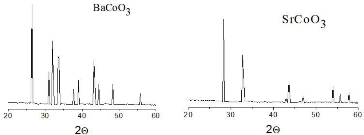
Figure 1: shows X-ray patterns of barium and strontium perovskite cobaltites.
