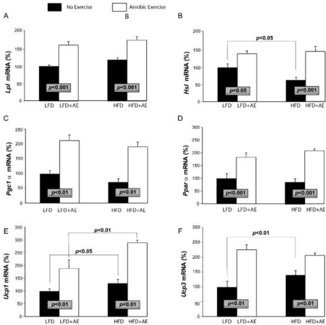
A) Lipoprotein lipase ( Lpl ) mRNA. B) Hormone-sensitive lipase ( Hsl ) mRNA. C) Peroxisome proliferator-activated receptor-gamma coactivator alpha ( Pgc1 α ) mRNA. D) Peroxisome proliferator-activated receptor alpha ( Ppar α ) mRNA. E) Uncoupling proteins 1 ( Ucp1 ) mRNA. F) Uncoupling proteins 3 ( Ucp3 ) mRNA. The results were expressed as a mean ± standard error (S.E.M.). Two-way ANOVA, followed by Tukey's multiple comparisons test, was carried out. p values are embedding in figures. n =8 per group. Black columns - sedentary animals. White columns - trained animals. Low Fat Diet (LFD), High fat Diet (HFD, Aerobic exercise (AE)).
