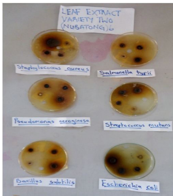
Figure 6: Plate 9- Zone of inhibition of Canarium schweinfurthii leaf extracts from Nubatong village and the control
